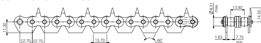
Attachment type 150
