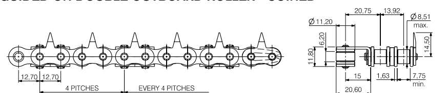
Attachment type 150
