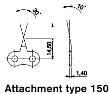
Attachment type 150
