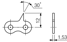
Attachment type 167
