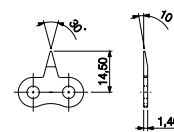
Attachment type 150
