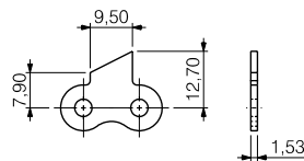
Attachment type 163
