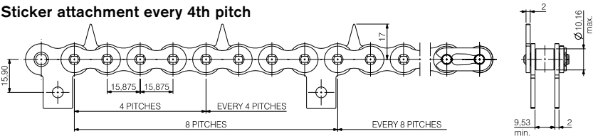
Attachment type 177
