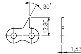
Attachment type 177
