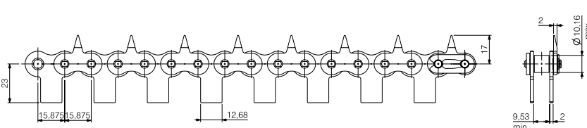
Attachment type 190
