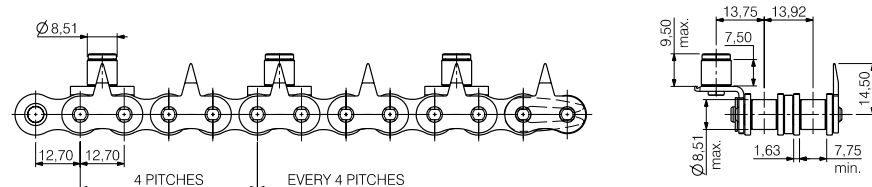
Attachment type 150
