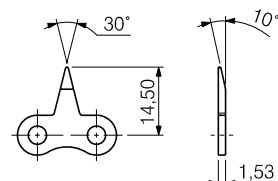
Attachment type 141
