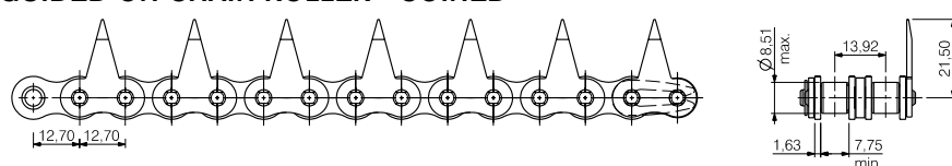
Attachment type 1010
