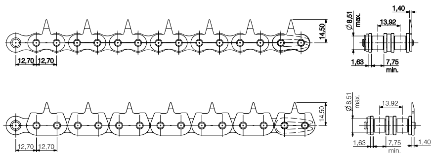
Attachment type 150
